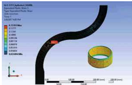
Expansion Joint Design
