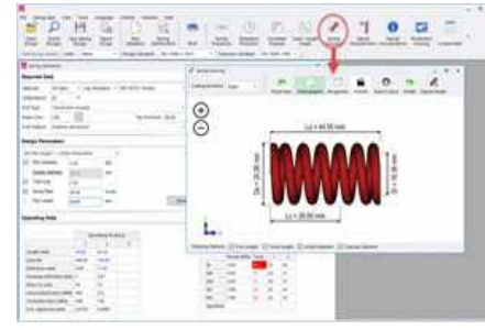
Customized Spring Design
